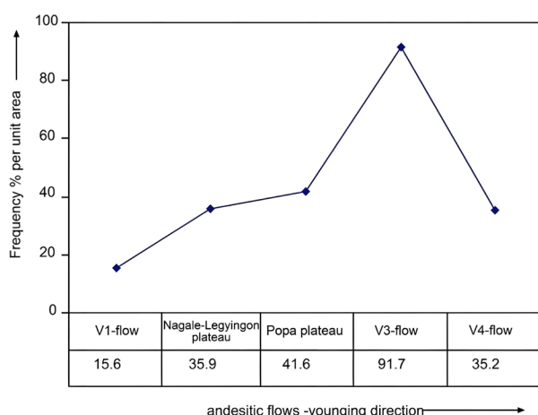
Figure 6. Mafic phenocryst distribution histogram of different andesitic flows in Mount Popa area.
