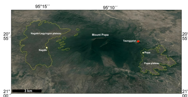
Figure 10. Satellite image showing Mount Popa volcanic cone and Plateaux of Popa plateau and Nagale-Legyngon plateau, (Looking South).
