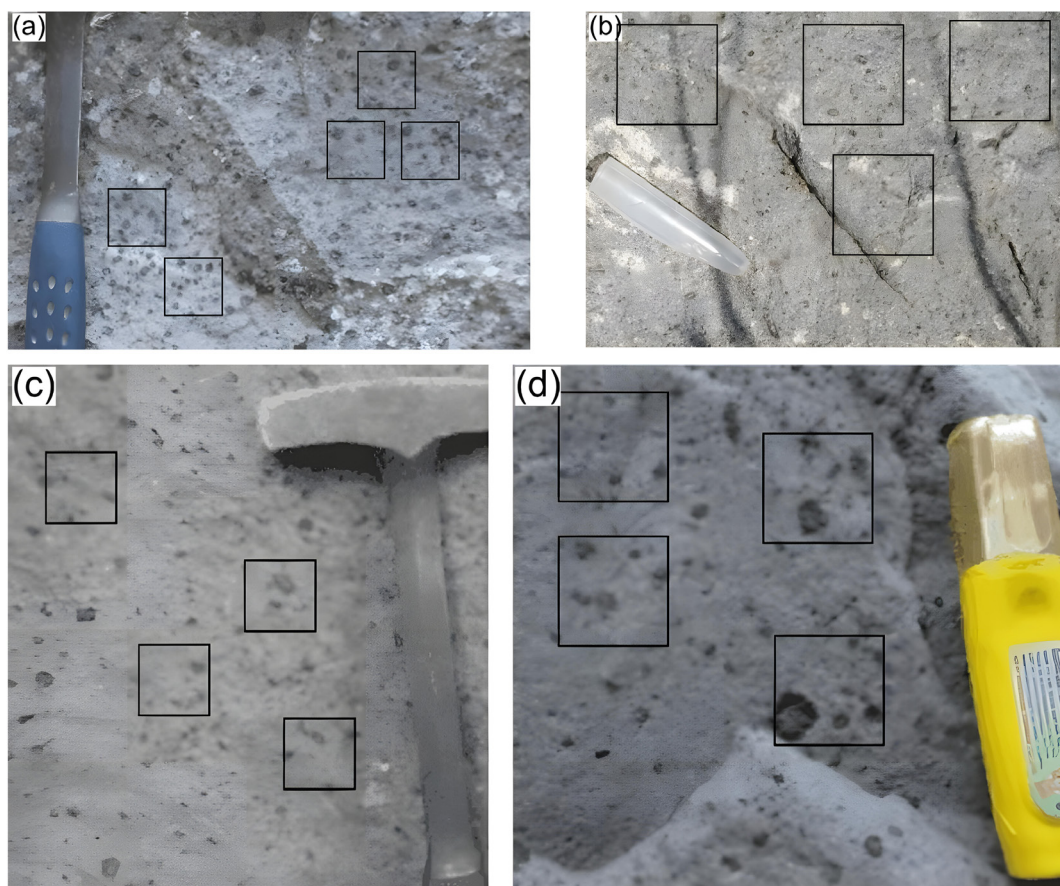
Figure 5. Photographs showing the demarcated one-unit area (1 inch x 1 inch) to be counted on the surface of different andesitic flow samples. (a). Popa plateau andesite, (b). Nagale-Legyngon plateau andesite, (c), V1 flow andesite, (d). V4 flow andesite.
