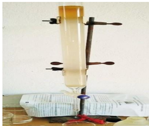
Figure 3. Column chromatography
