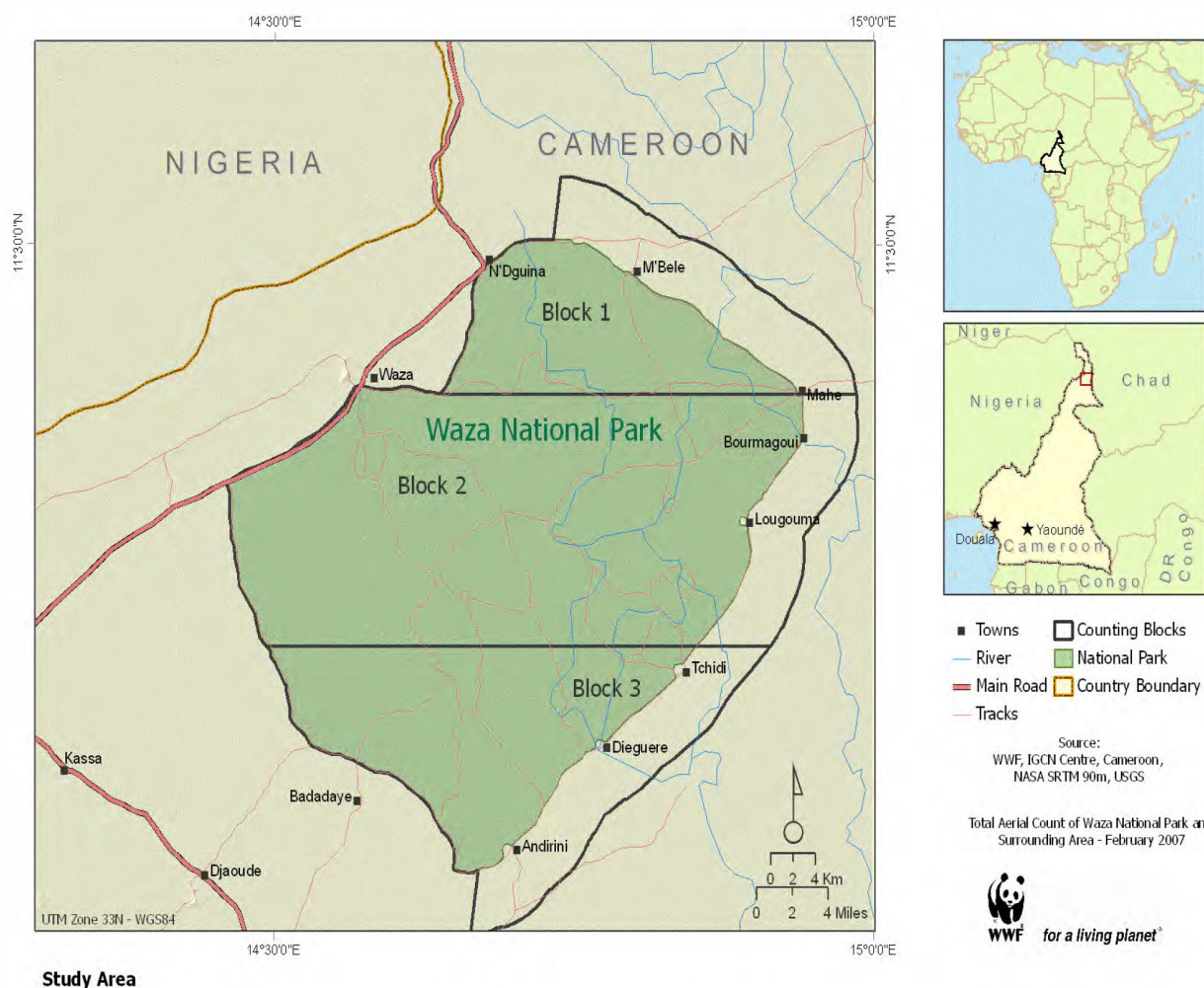
Figure 1. The map of Waza National Park, Cameroon [39].
