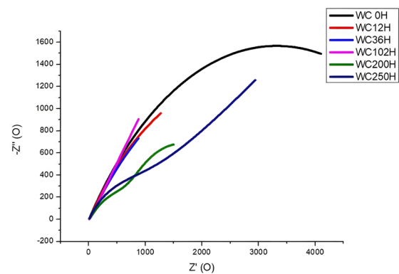
Figure 13. Nyquist plot for the WC-10Co-4Cr coating ( Z(O) = \text{ohm.cm}^2 ).
