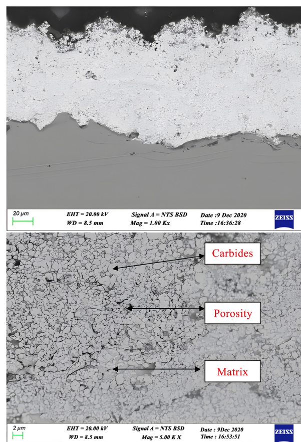
Figure 5. FESEM microstructure of WC-10Co-4Cr coating.
