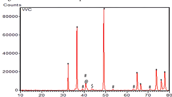
Figure 2. XRD spectrum of the WC-10Co-4Cr coating on AISI304 stainless steel. *, #, @, $ represents WC, W_2O , Co 6 W 6 C, Co 3 W 3 C phases respectively.
