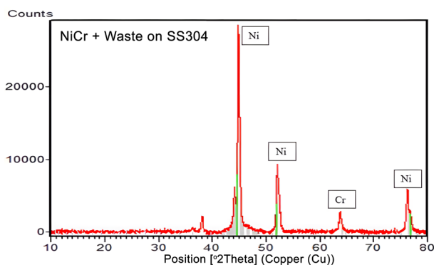
Figure 4. XRD spectrum of the NiCrIW coating on AISI304 stainless steel.
