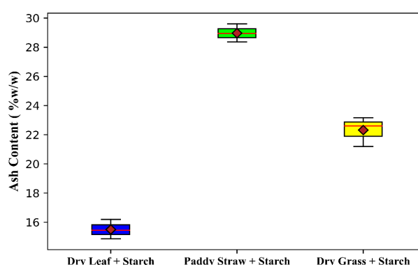
Figure 6. Effect of biomass briquettes on ash content.
