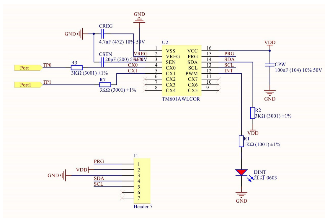
Figure 3. Hardware circuits of the sensor module.
