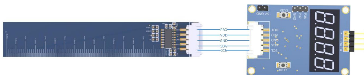
Figure 5. Calibration of the liquid level sensor.
