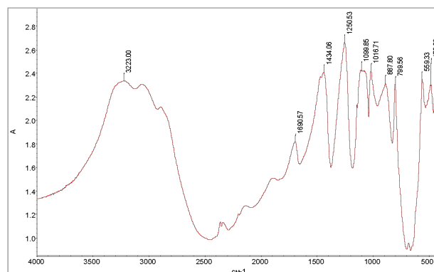
Figure 11. The IR spectrum of APP.
