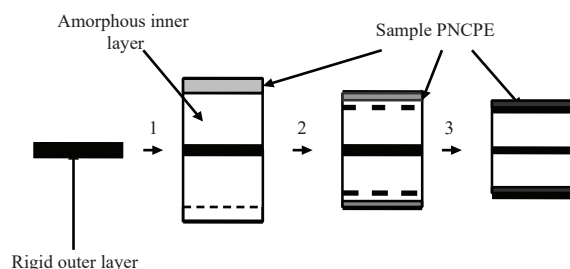
Figure 17. Char formation diagram on the surface of PNCPE.
