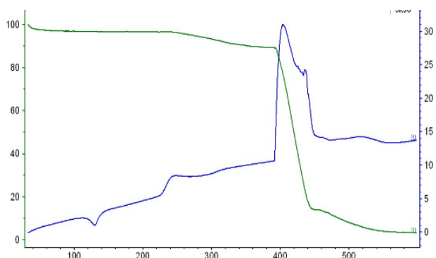
Figure 2. TGA and DSC curves of ZBPPE.
