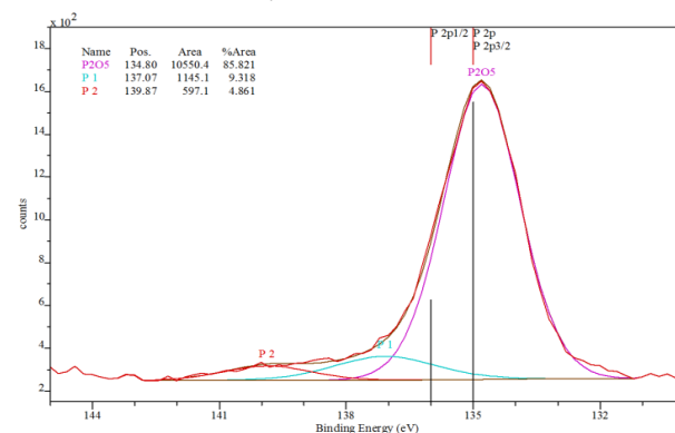
Figure 10. XPS P2P line of the PNCPE inner layer of the char.
