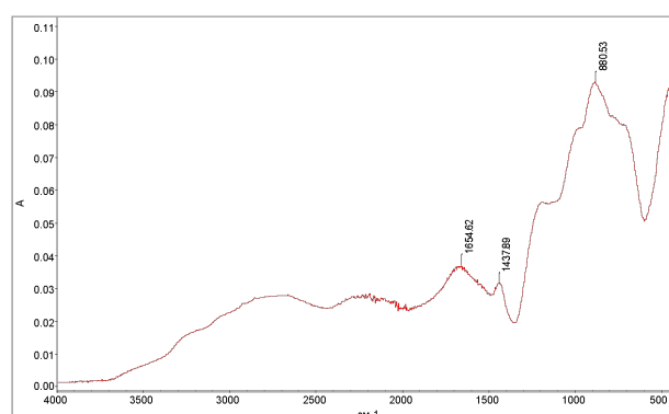
Figure 12. IR spectrum of APP after heating at 600\text{ }^{\circ}\text{C} .
