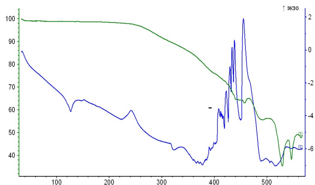
Figure 3. TGA and DSC curves of PNCPE.
