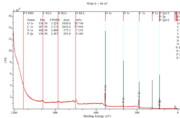
Figure 9. XPS spectra of the PNCPE outer layer of the char.
