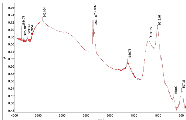
Figure 15. IR spectrum of APP+PER after heating at 600 °C.
