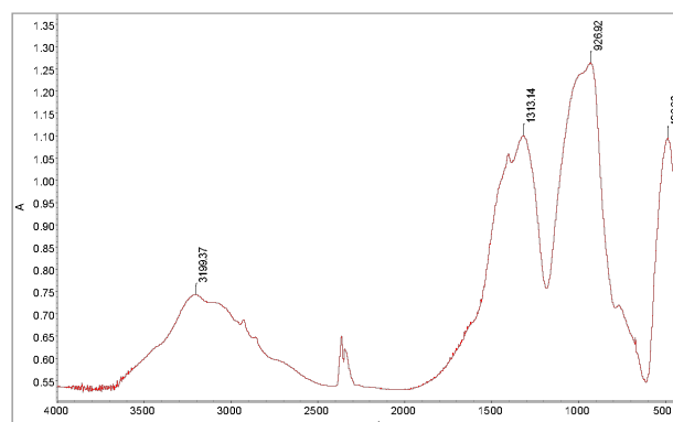
Figure 14. IR spectrum of PNCPE after heating at 600\text{ }^{\circ}\text{C} (outer layer).
