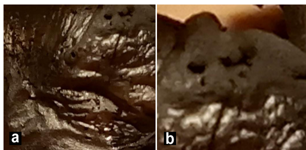
Figure 18. The surface of the char produced in oscillation mode (a) and without oscillation(b)
