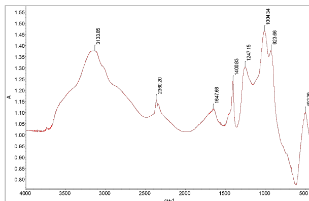
Figure 16. IR spectrum of APP+MEL after heating at 600 °C.
