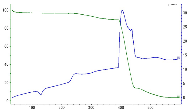
Figure 1. TGA and DSC curves of HDPE.
