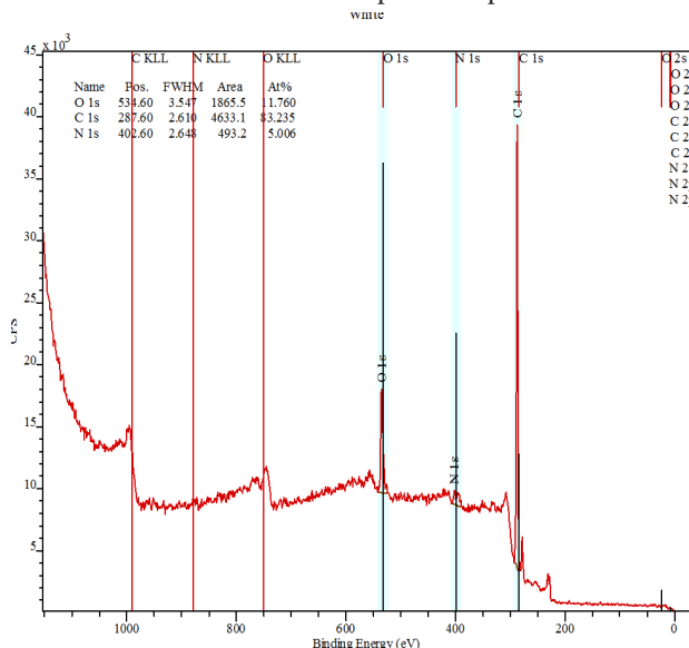
Figure 5. XPS spectra of ZBPPE.
