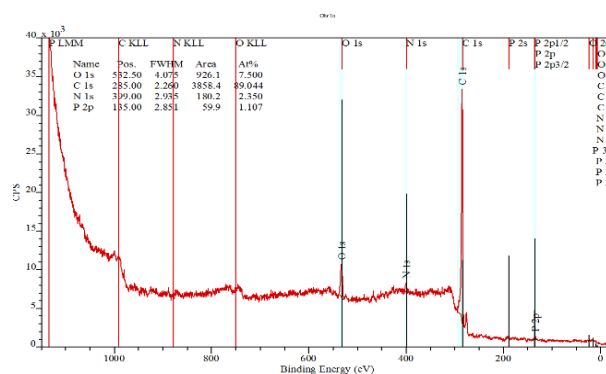
Figure 7. XPS spectra of the PNCPE inner layer of the char.
