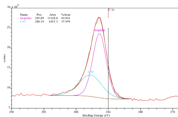
Figure 8. XPS C1s line of the PNCPE inner layer of the char
