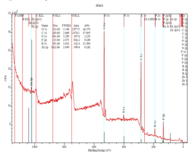
Figure 6. XPS spectra of the ZBPPE inner layer of the char.
