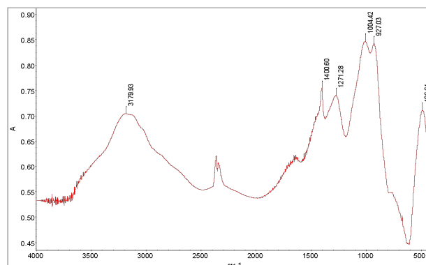
Figure 13. IR spectrum of PNCPE after heating at 600\text{ }^{\circ}\text{C} (inner layer).
